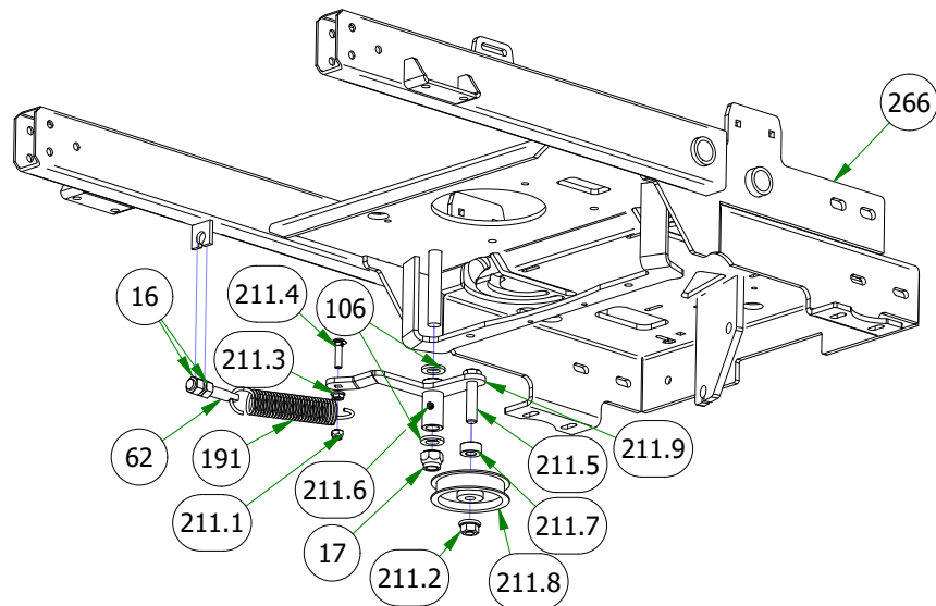
36" IDLER ARM ASSEMBLY
