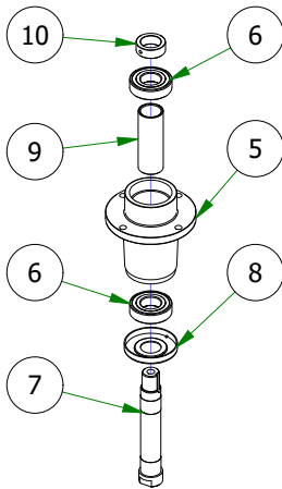
037-6015-50 Spindle- Aluminum -2012 ZT
