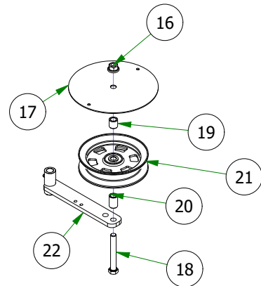
039-6945-20 2020 61 Revolt Deck Idler Assembly
