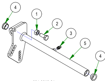
031-0053-21 2021 Maverick Drive Arm Actuator RH Assembly
